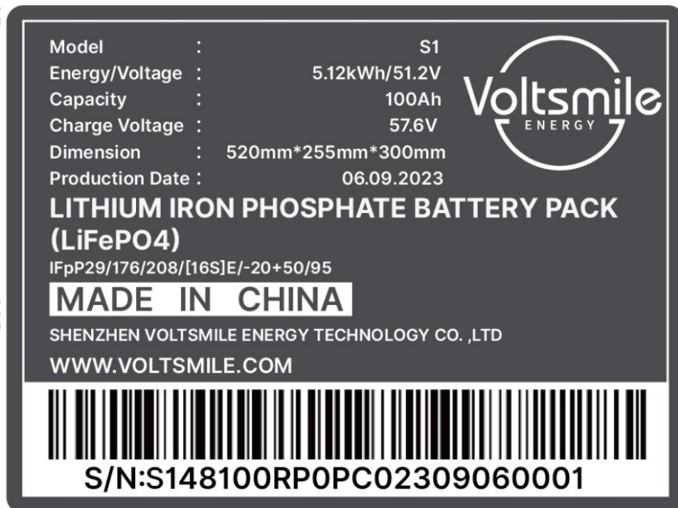
Figure 4 Battery Label
